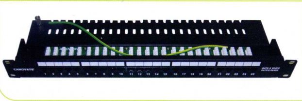
UTP 25 Port Horizontal Cat3 Patch Panel
